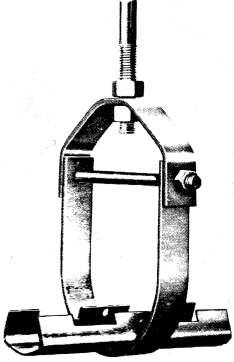
Fig 100S: Clevis Hanger with Welded Saddle
